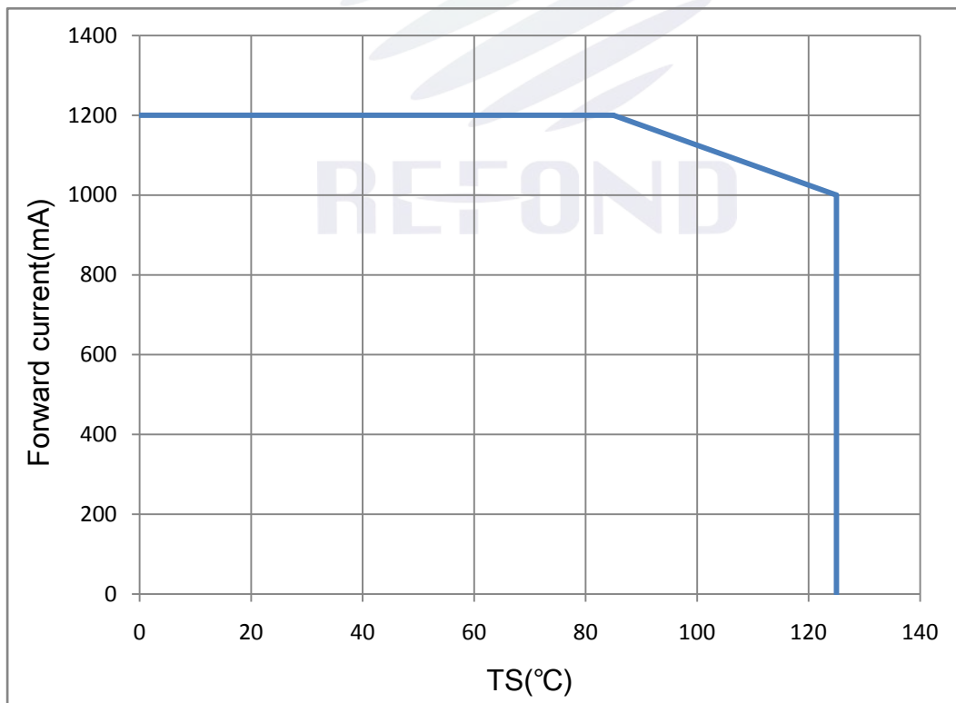
Fig. 1-10 Solder Temperature Vs Forward Current 管脚温度与正向电流特性曲线 T j ≤ 150°C
