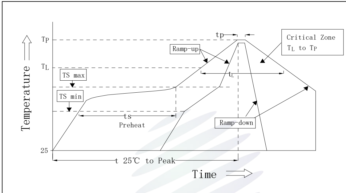
Fig.3-1 SMT Reflow Soldering Instructions SMT 回流焊说明
