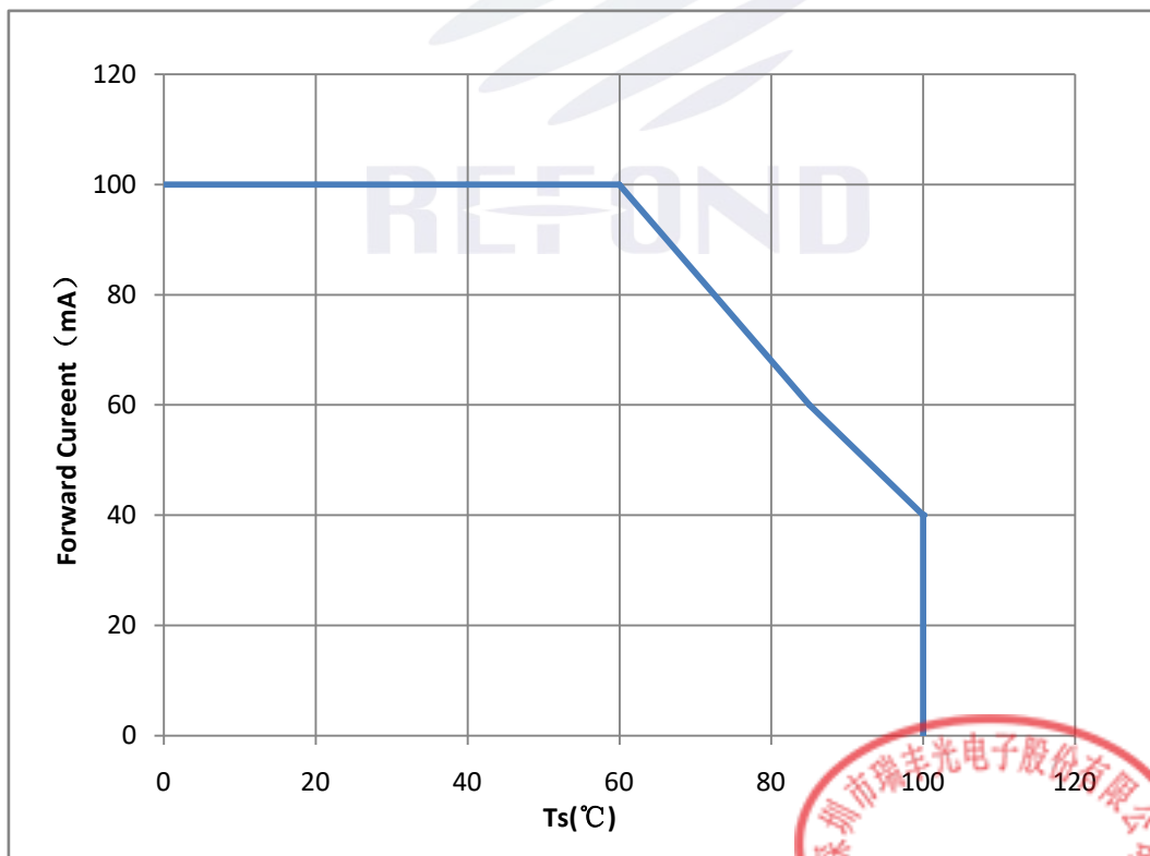
Fig. 1-10 Solder Temperature Vs Forward Current 管脚温度与正向电流特性曲线 Tj ≤ 120°C
